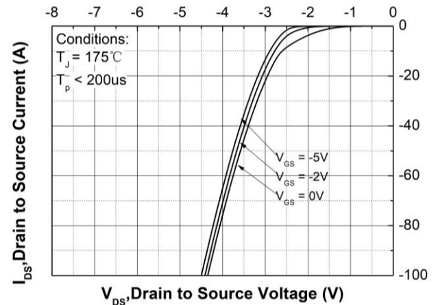
Figure 10. Body Diode Characteristic at T J = 175 °C
