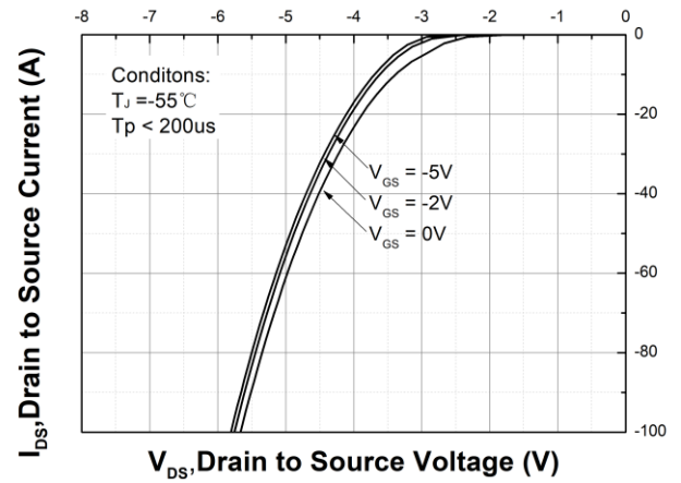
Figure 8. Body Diode Characteristic at T J = -55 °C
